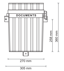
PDS/360
